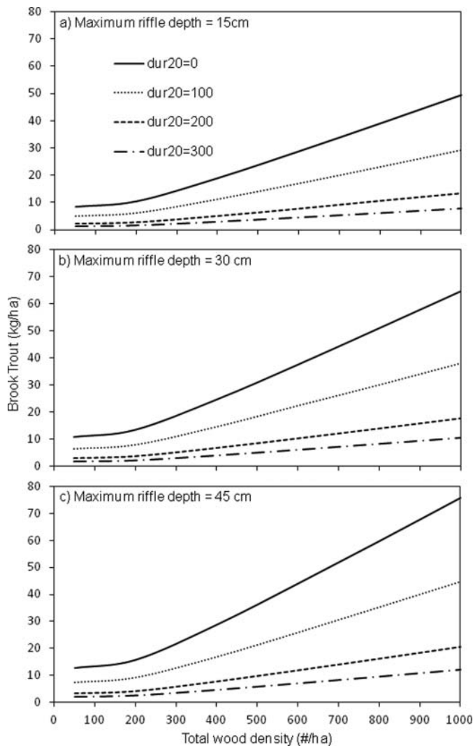
FIGURE 3. Brook Trout biomass predicted by the top-ranked model at various durations of water temperatures exceeding 20°C (dur20 [h]) and total wood densities at (a)–(c) three different maximum riffle depths.
