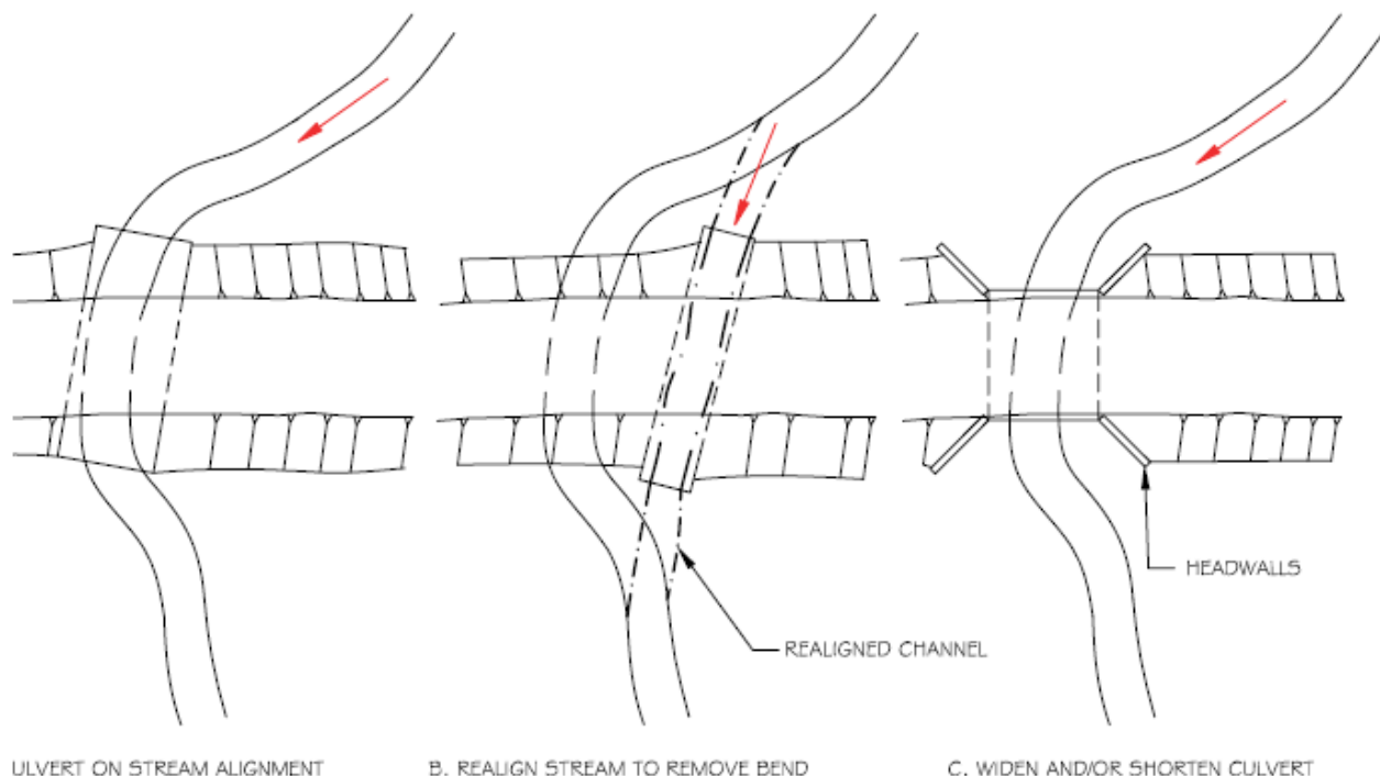
Figure 9.4: Options for locating a culvert on a bend, see text (Forest Service Stream-Simulation Working Group 2008).
