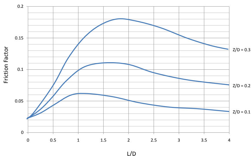
Figure 6.2: Variation of Darcy Weisback friction factor with baffle spacing.
